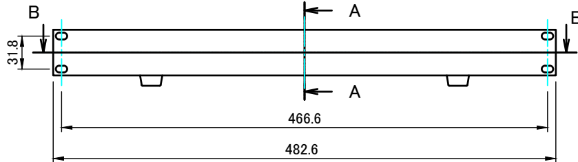
F view
