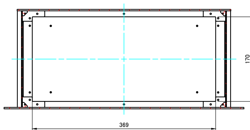
B-B (1:4.5)
