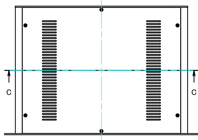
E view
