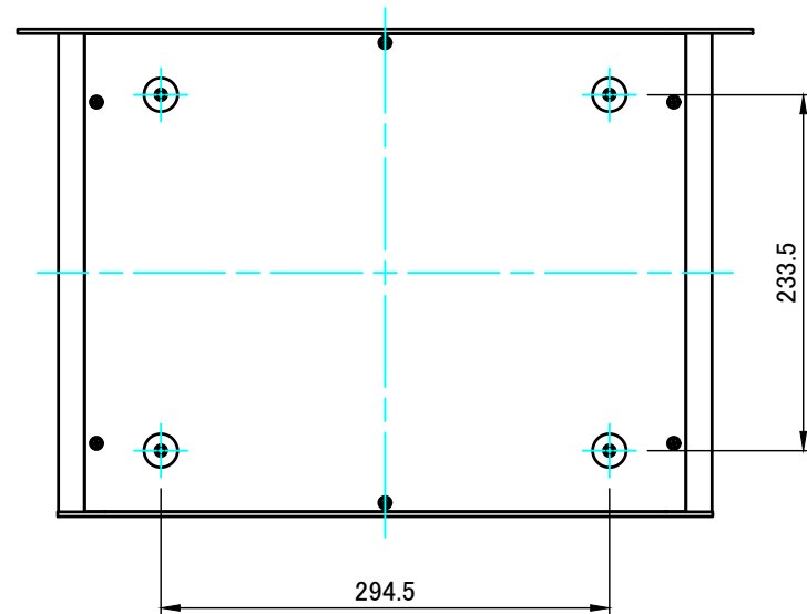
F view
