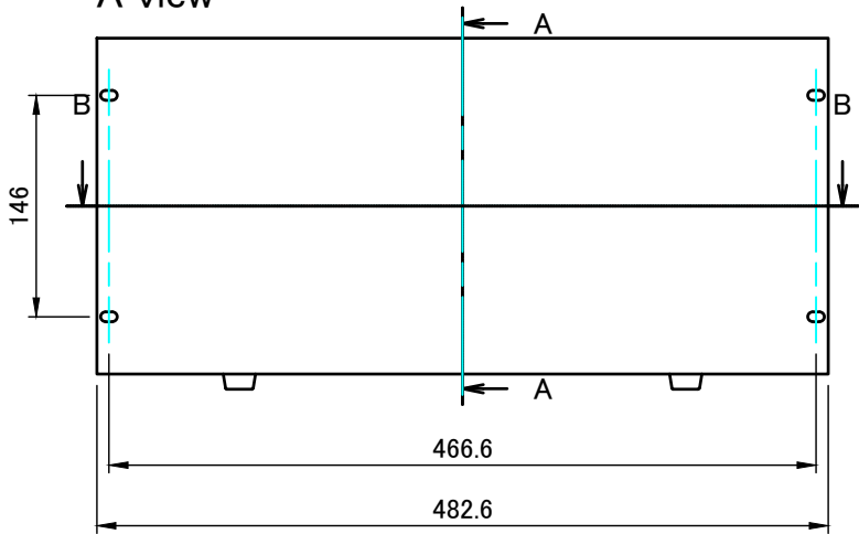
A view
