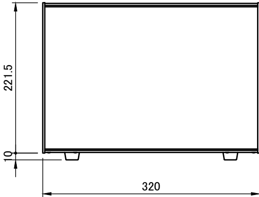
C view
