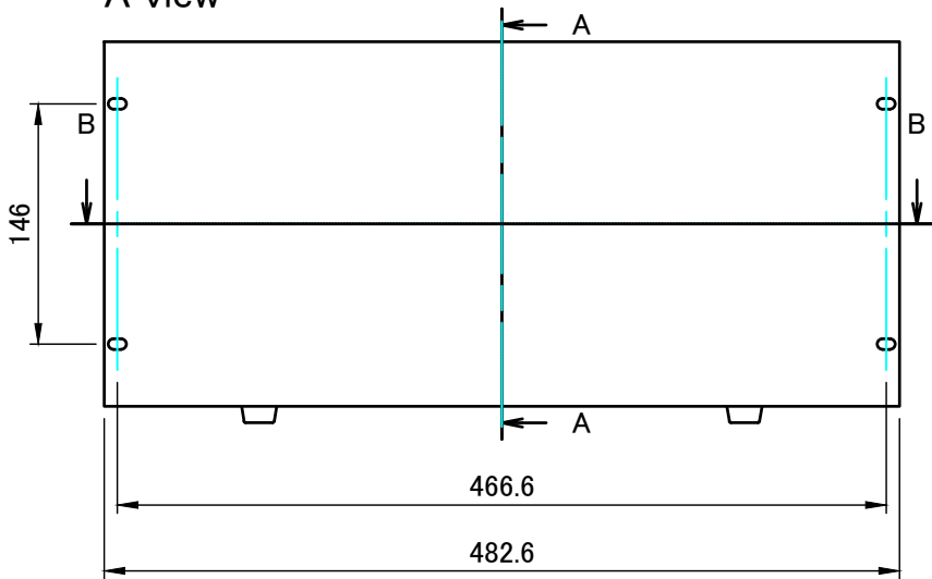
A view
