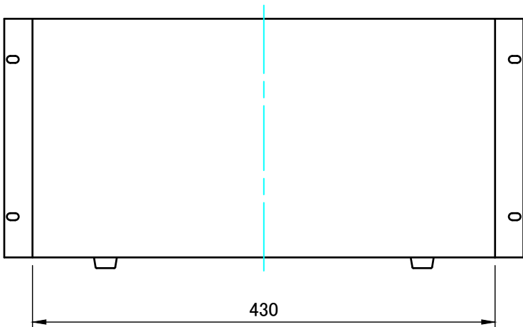
B view
