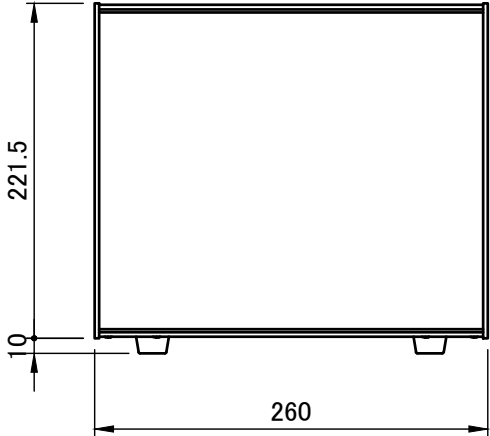
C view
