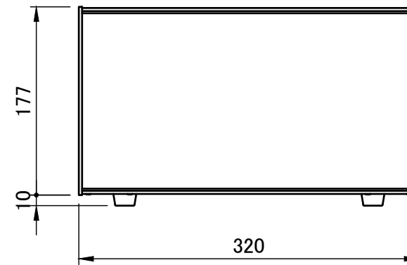
C view
