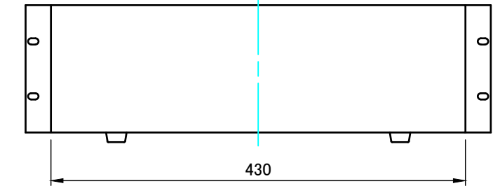
B view
