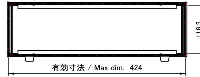
A-A (1:5.5)
