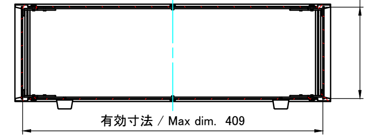
C-C (1:5)
