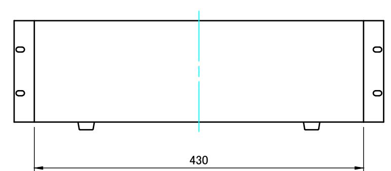
B view
