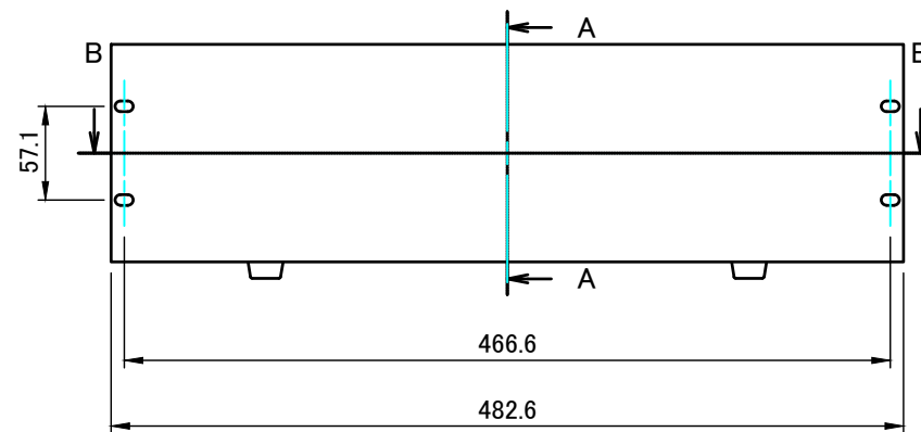
F view
