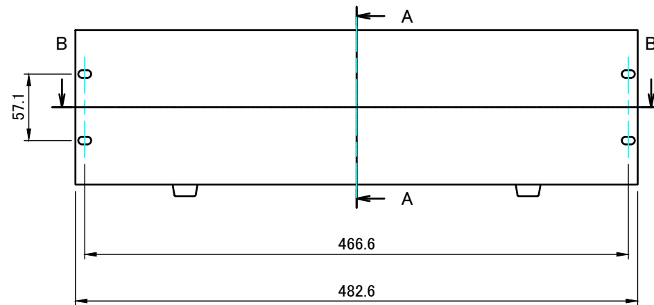
F view
