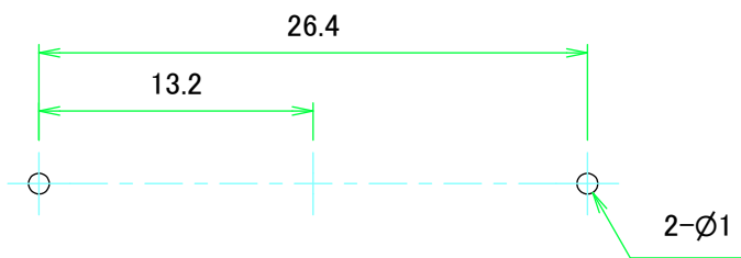
推奨基板加工寸法 Recommended PCB hole layout
