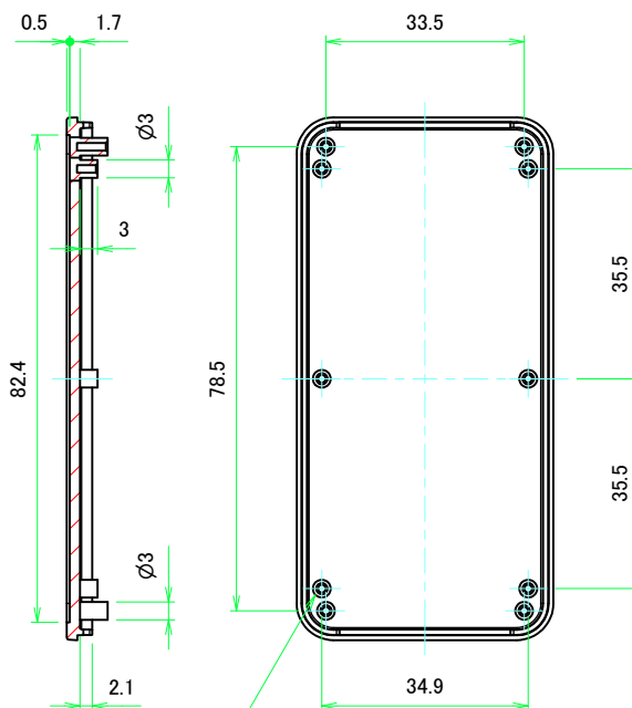
C-C (1:1)
