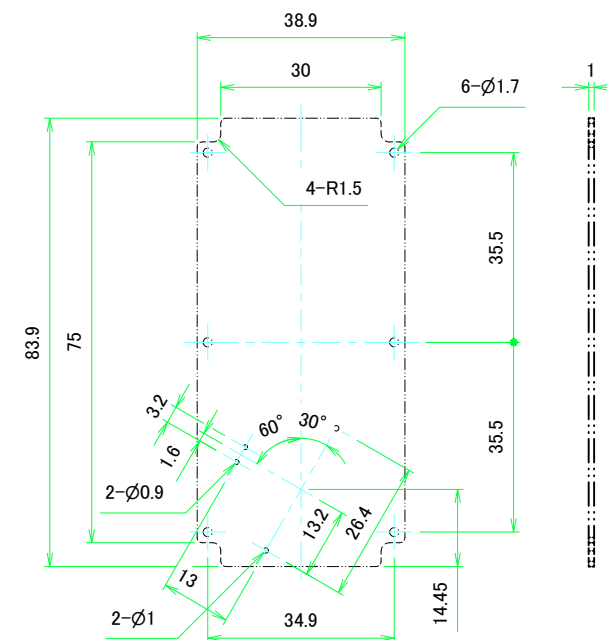
推奨基板形状 / Recommended PCB dimension
