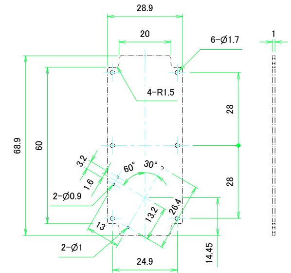
推奨基板形状 / Recommended PCB dimension
