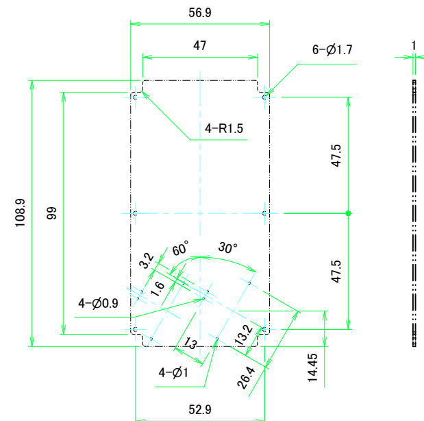
推奨基板形状 / Recommended PCB dimension
