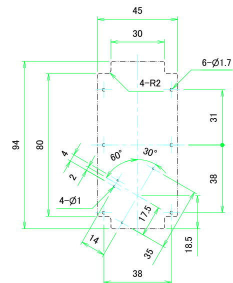
推獎基板形狀 / Recommended PCB dimension
