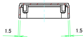
F-F (1:1.5)
