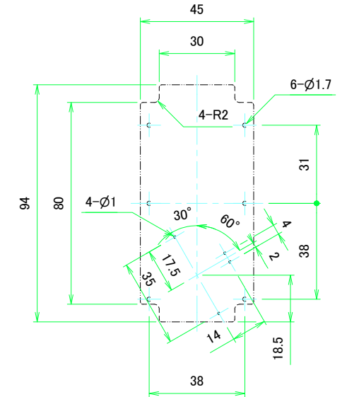
推奨基板形状 / Recommended PCB dimension
