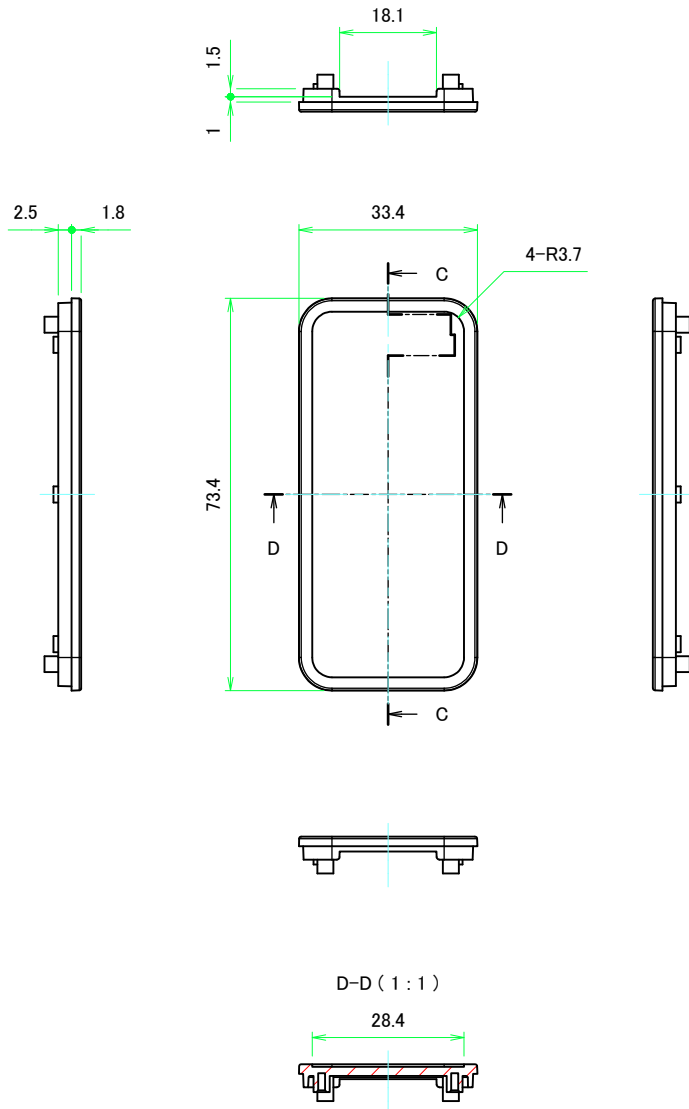
C-C (1:1)
