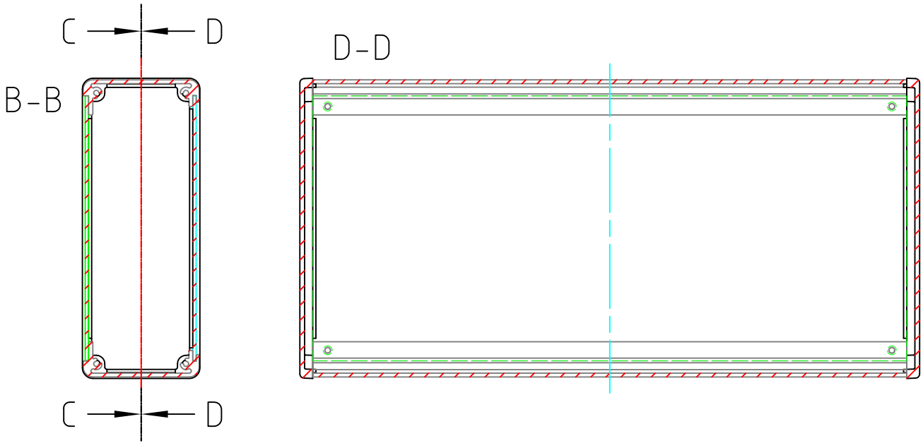
ネジ止めパネル(内視) / Screwed panel (Internal View)
