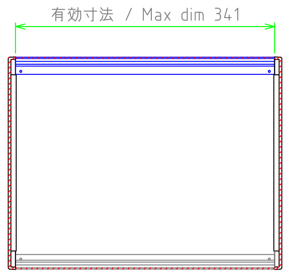
ネジ止めパネル(内視) Screwed panel (Internal View)
