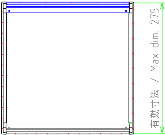
ネジ止めパネル(内視) Screwed panel (Internal View)
