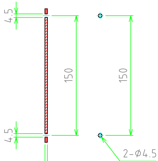
板厚 t1.8~t4.0 Mountable thickness t1.8~t4.0
