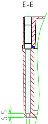
φ 4.3 外部取付用穴 External mounting holes
