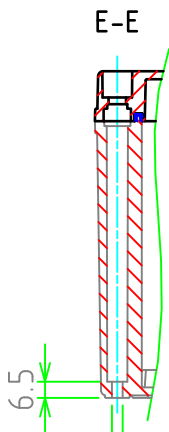
φ 4.3 外部取付用穴 External mounting holes
