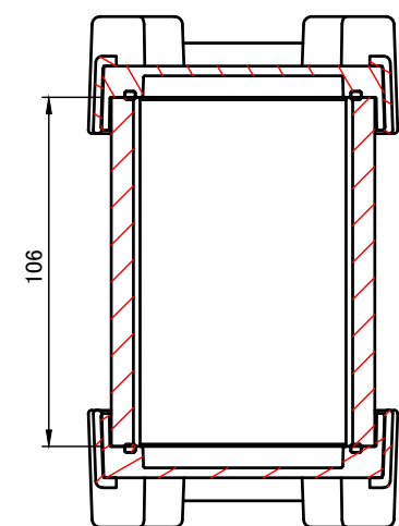
C-C (1:2.5)
