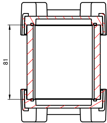
C-C (1:2.5)
