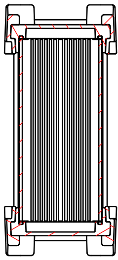
B-B (1:3)
