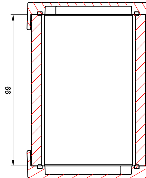
C-C (1:1.5)
