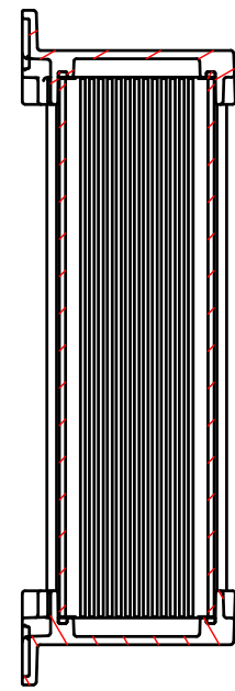
B-B (1:3)
