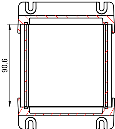
C-C (1:2.5)
