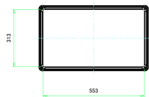
C-C (1:8.5)
