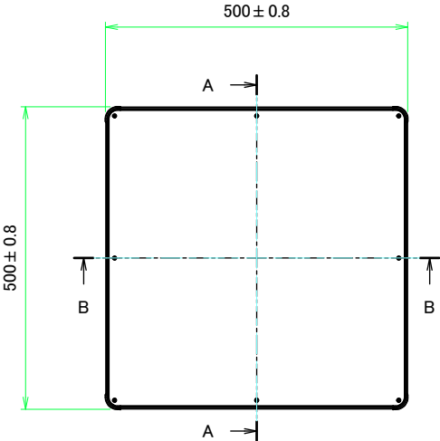
E view
