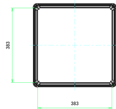
C-C (1:7)
