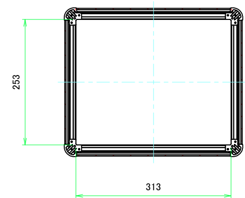
C-C (1:5.5)
