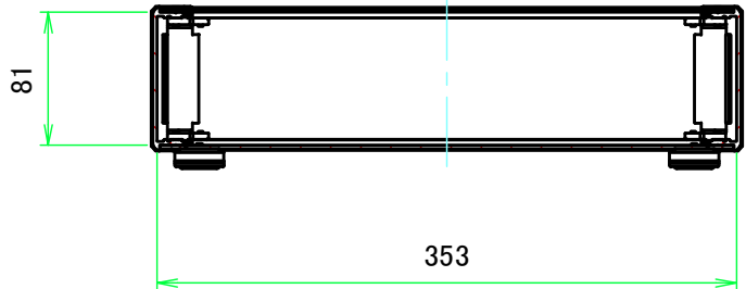
B-B (1:5)
