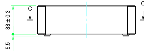
B-B (1:5)
