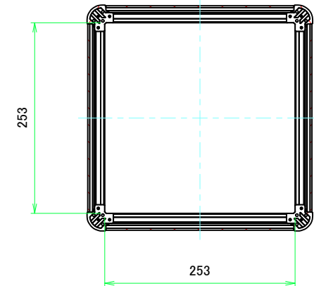
C-C (1:5)
