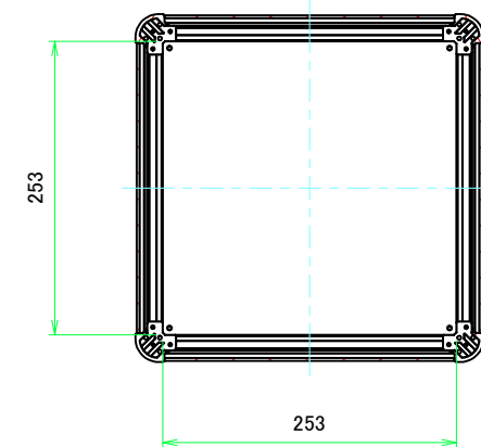
C-C (1:5)
