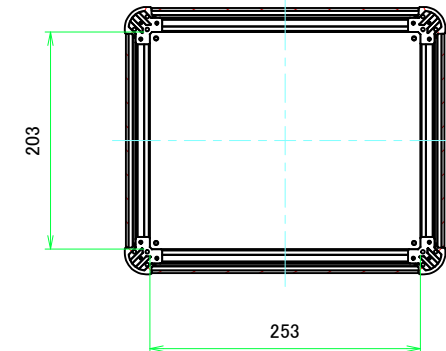
C-C (1:5)
