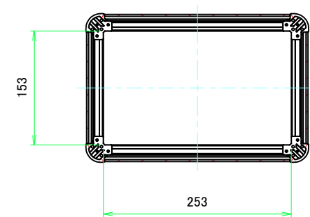
C-C (1:5)
