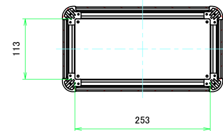
C-C (1:5)
