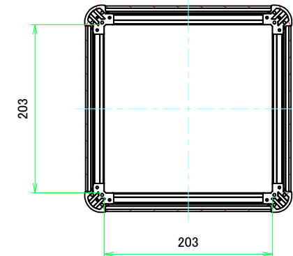
C-C (1:4.5)
