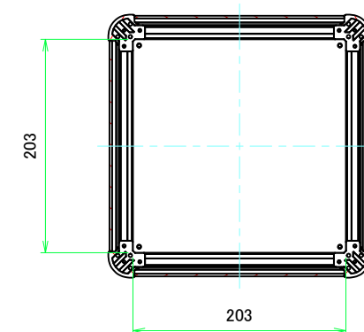
C-C (1:4.5)
