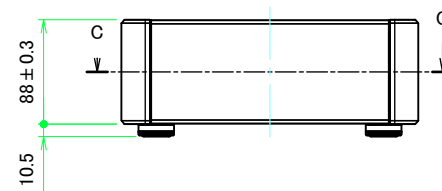
B-B (1:4.5)
