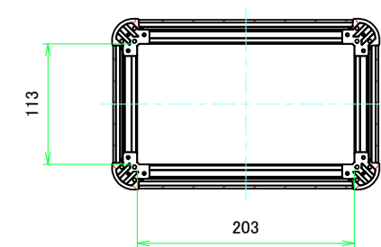
C-C (1:4.5)
