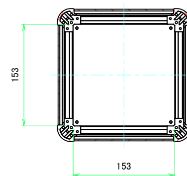
C-C (1:4)
