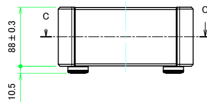
B-B (1:4)
