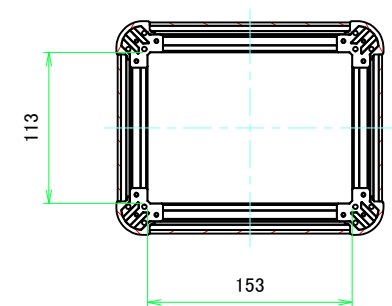
C-C (1:4)
