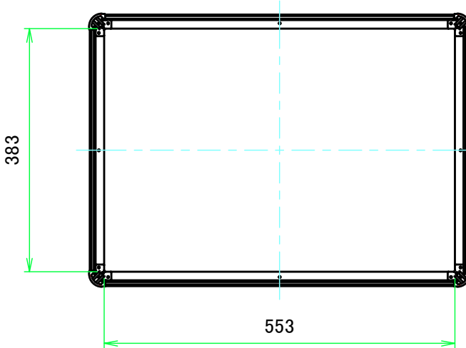
C-C ( 1:8.5 )
