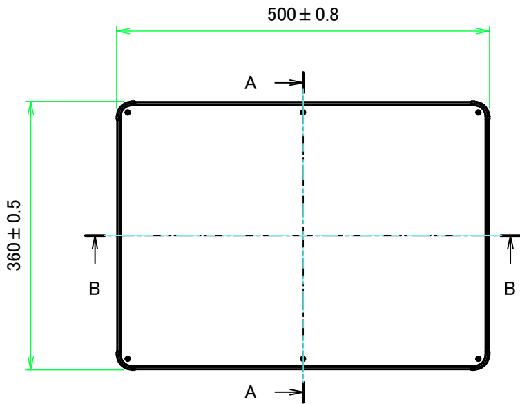
E view
