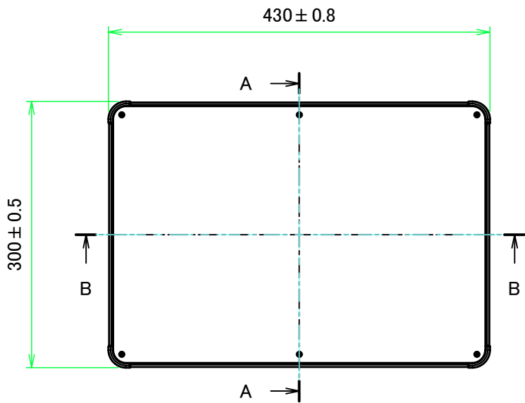
E view
