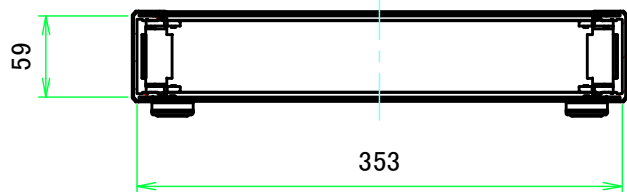
B-B ( 1:5.5 )
