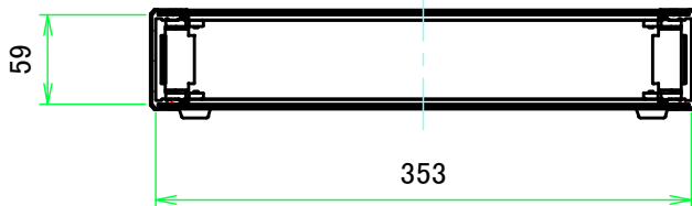
B-B ( 1:5.5 )
