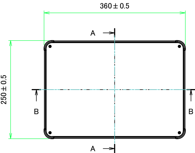
E view
