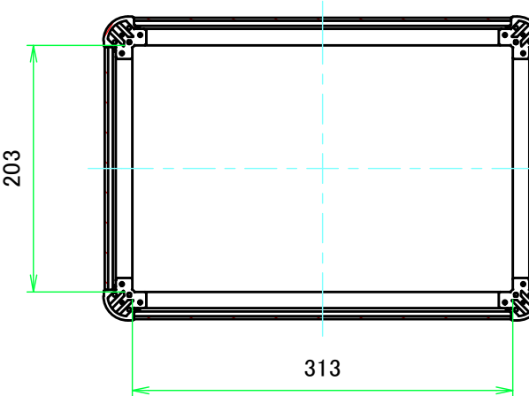
C-C ( 1:5.5 )
