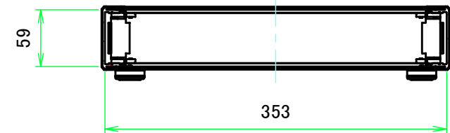
B-B ( 1:5.5 )
