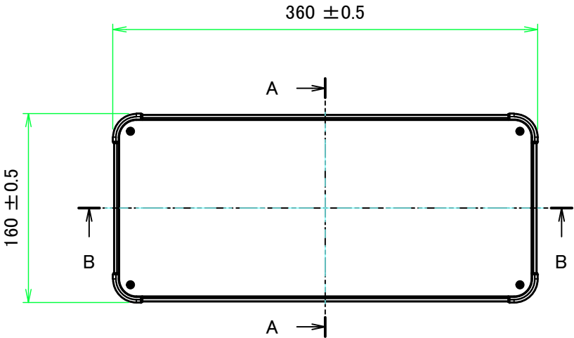
E view
