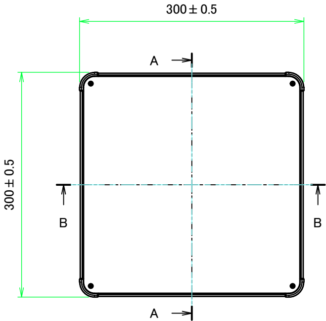
E view
